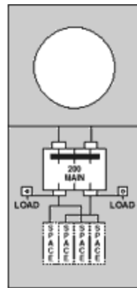
Service Entrance 200 Amp Ringless Pedestal 331-522 200 Amp
